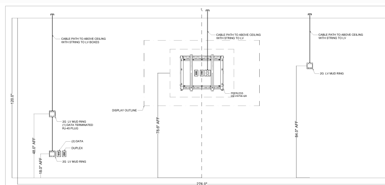
1 INFRASTRUCTURE WALL ELEVATION SCALE: 1" = 1'
