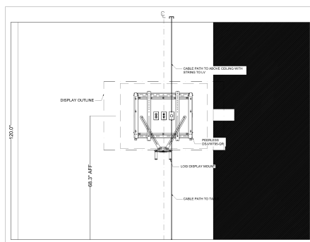
1 INFRASTRUCTURE WALL ELEVATION SCALE 1/4" = 1'-0"
