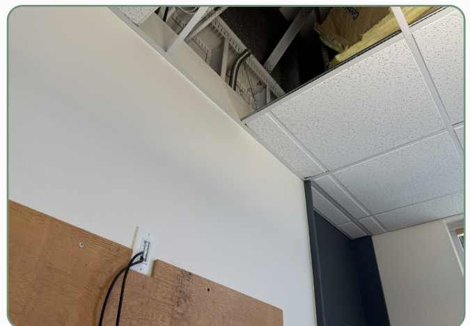
WALL AND CEILING COORDINATION | IN PROGRESS
