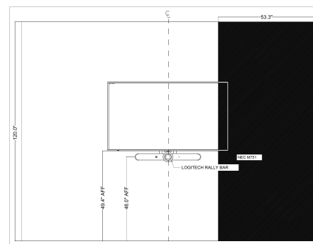
2 DEVICE WALL ELEVATION SCALE 1/4" = 1'-0"
