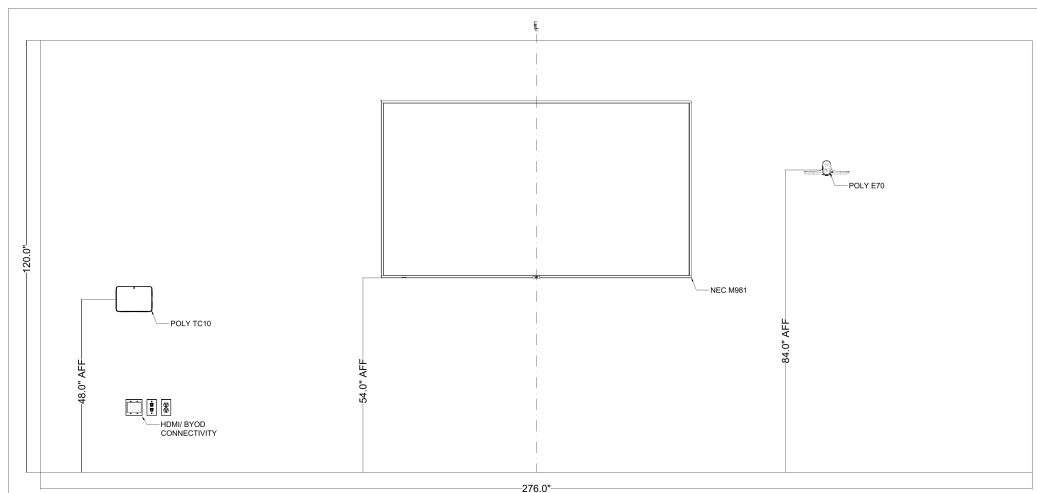
1 DEVICE WALL ELEVATION SCALE: 1" = 1'
