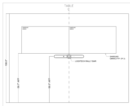
1 DEVICE ELEVATION SCALE 1" = 1/2"
