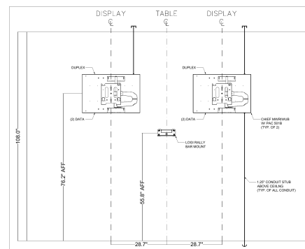
2 INFRASTRUCTURE ELEVATION SCALE 1" = 1/2"
