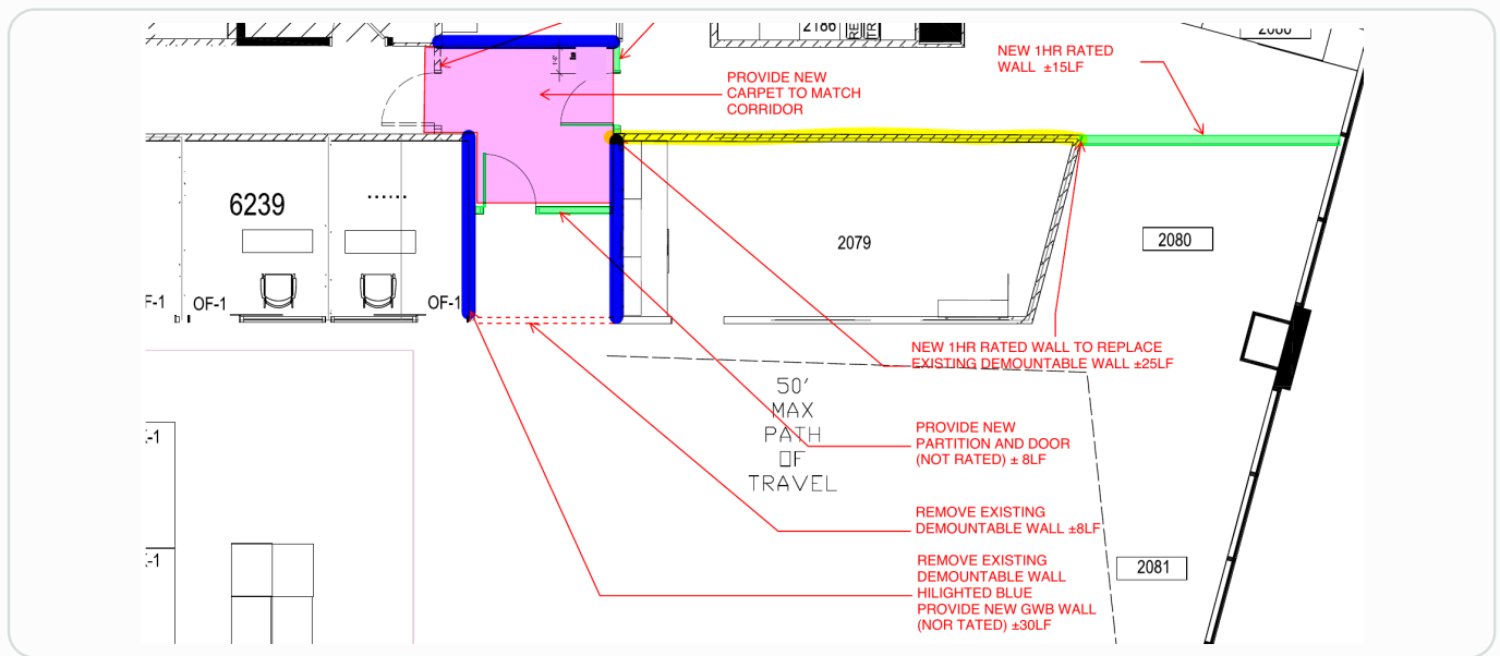
ARCHITECTURAL DEMISING AND PARTITION SCOPE DETAIL
