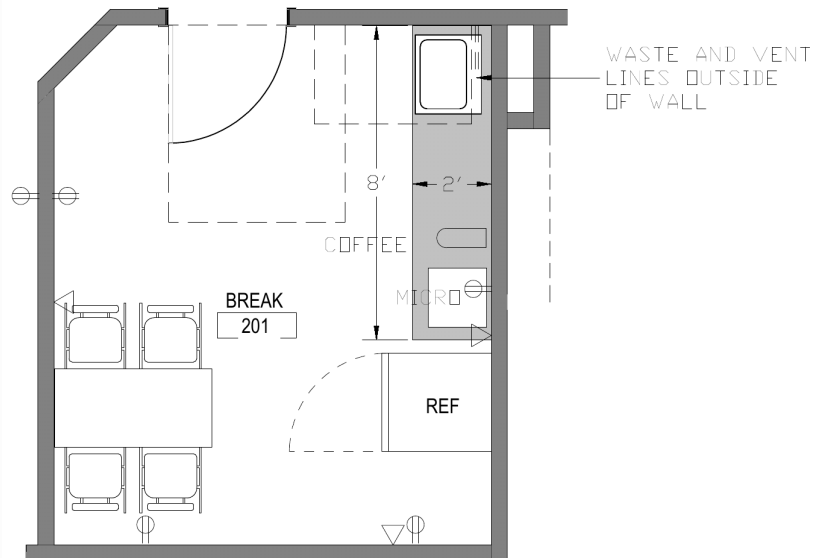
KITCHENETTE ROOM AND SERVICE-PLANNING LAYOUT
